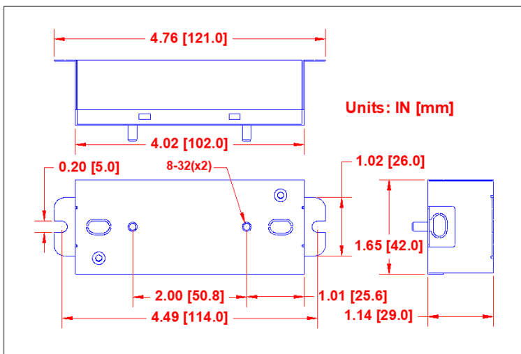
M28-XM & M38-XM Series : 4.76" x 1.65" x 1.14"
