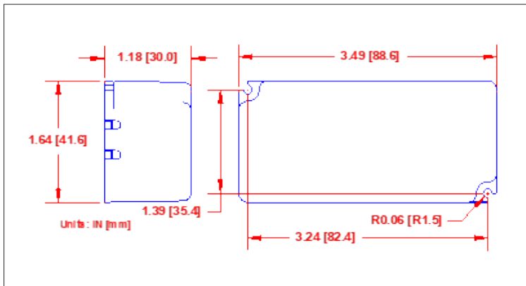
QM40 Series : 88.6 x 41.6 x 30mm
