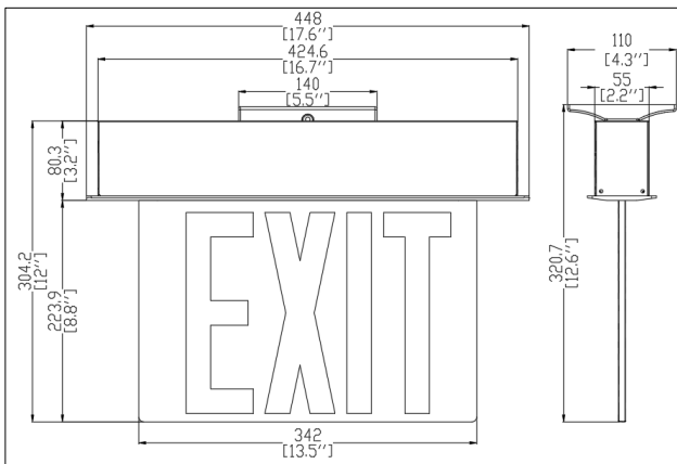
8" Surface mount (top) size
