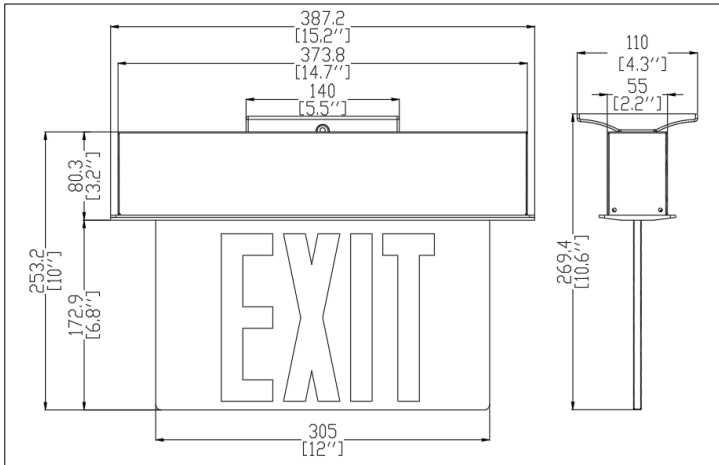
6" Surface mount (top) size
