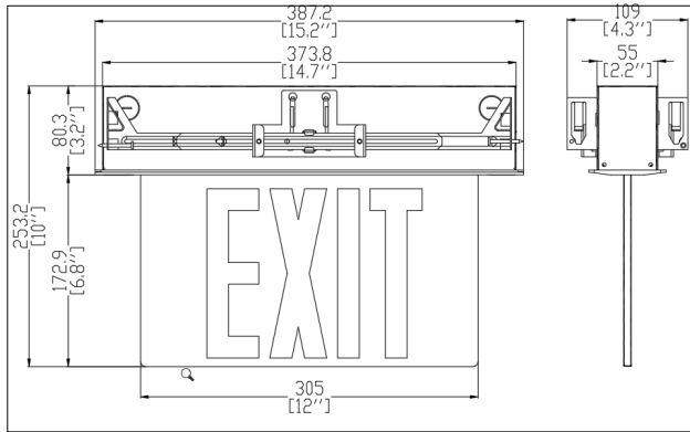
6" Full recessed mount (top) size
