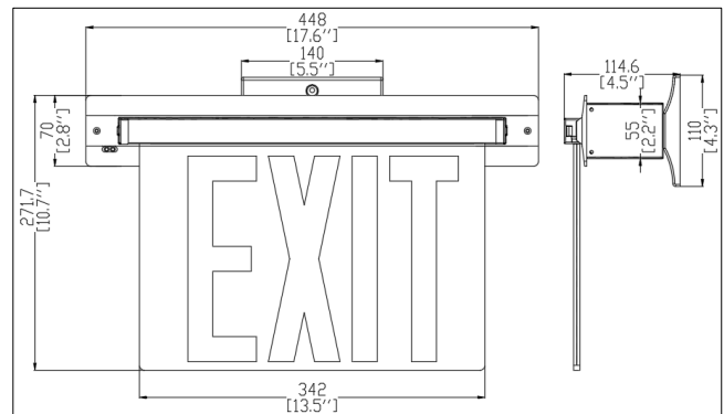
8" Surface mount (wall) size
