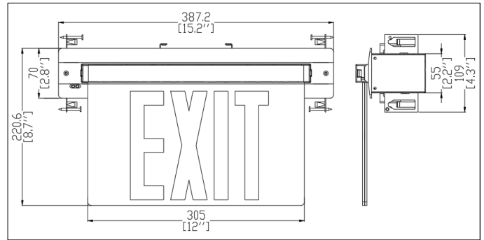
6" Full recessed mount (wall) size
