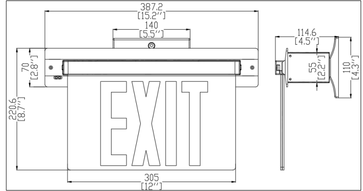
6" Surface mount (wall) size
