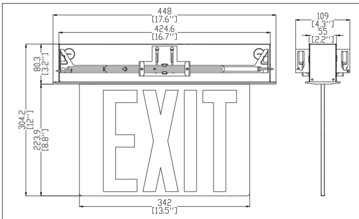
8" Full recessed mount (top) size
