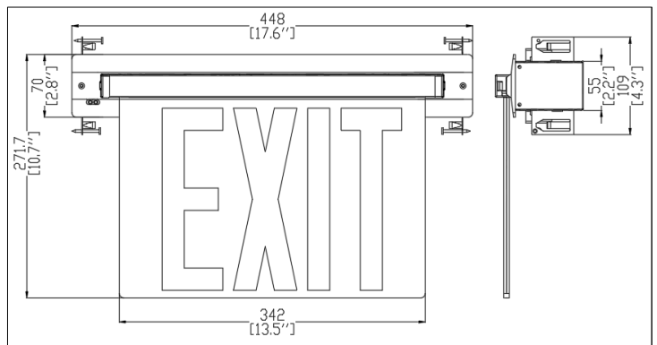
8" Full recessed mount (wall) size
